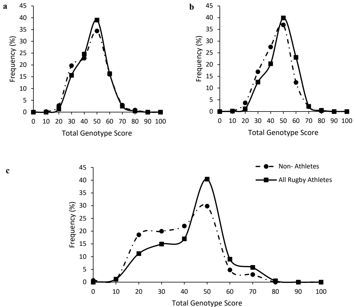
Figure 1. Frequency distribution of TGS based on; a: Prior literature as calculated from Table 1 (Model 1) Mean (SE) kurtosis statistics in all rugby athletes were -0.063 ( 0.201 ) and non-athletes was -0.130 ( 0.233 ). b: Elite rugby athlete data as calculated from Supplementary Material Table 1 (Model 2). Mean (SE) kurtosis statistic in all rugby athletes was -0.320 ( 0.201 ) and non-athletes was 0.096 ( 0.233 ). c: SNPs previously associated with elite status in rugby as calculated from Supplementary Material Table 2 (Model 3) Mean (SE) kurtosis statistic in All rugby athletes was -0.161 ( 0.201 ) and non-athletes was 0.296 ( 0.233 ). Non-athletes ( n = 436 ), All rugby athletes ( n = 589 ).
