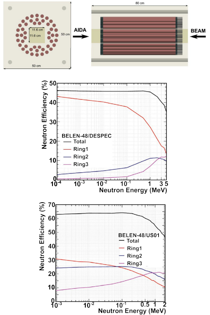
Fig. 9. Upper panel: Schematic of the cross and lateral section of polyethylene matrix where the {}^3\text{He} proportional counters are shown in red. Middle/lower panels: Neutron detection efficiency for BELEN-48 detectors up to 5 MeV, obtained by Monte Carlo simulations with MCNPX, in the standard configuration (middle) and optimised for low Q_{\beta n} windows (lower). See text for details.
