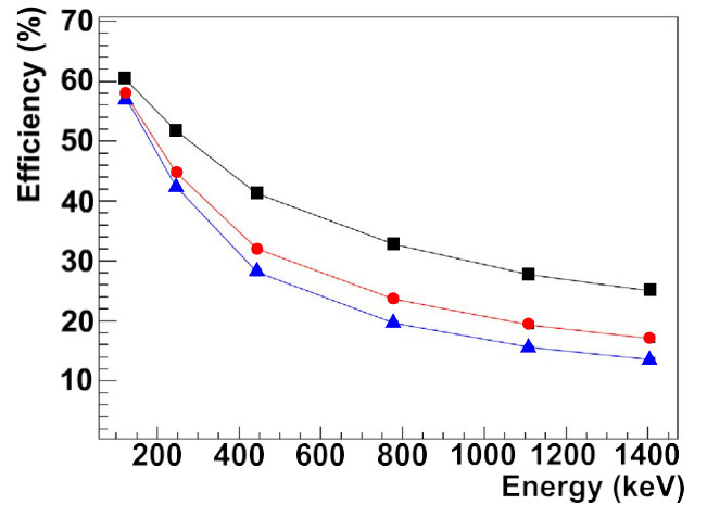
Fig. 7. Simulated peak efficiency for DEGAS as function of the \gamma -ray energy. The three lines correspond to Ge single crystal (blue triangle), Ge triple Cluster (red circles) and Ge calorimeter (black squares) add-back modes. The red option is the one implemented in the experiments, while the last one corresponds to summing of the energies of all responding crystals of the array.
