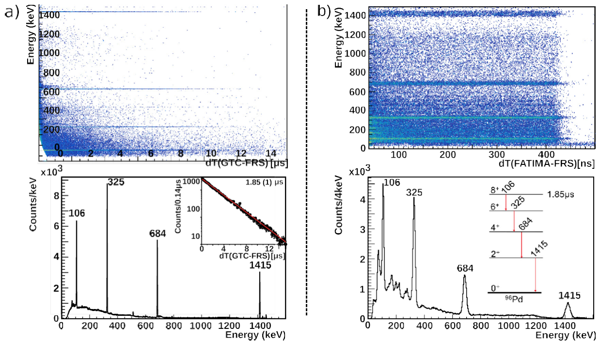
Fig. 14. (a) Prompt GTC spectra obtained during Exp.# 2 correlated with ^{96}\text{Pd} ions in the FRS. Top: Energy vs. time difference between signals from the GTC and from the S4 scintillator in the FRS. ( >2 counts/bin for clarity). Bottom: Projected \gamma -ray energy spectrum from top, in the inset the half-life extracted of 1.85(1) \mu\text{s} after gating on the 106, 325, 684 and 1415 keV \gamma -ray lines. (b) Same as (a) but for FATIMA. Note that the short collection time window for FATIMA restricts the ability to extract the \approx 2 \mu\text{s} isomer decay half-life for this particular study. The level scheme collated in [61] is shown as an inset in the lower panel of (b).
