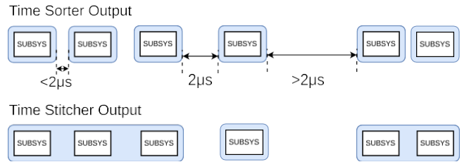
Fig. 13. Schematic of the ucesb time-stitching algorithm. Events from subsystems occurring less than a defined time (normally 2\mu s ) from the previous event are grouped together. Events themselves are unmodified.
