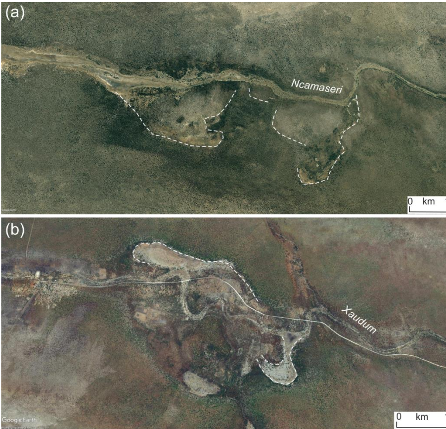
Figure 4: Abandoned meanders (dashed line) along the course of the (a) Ncamaseri and (b) Xaudum dry valleys in northwest Botswana. See Figure 1 for locations of images. Images courtesy of Google Earth, dated (a) 6 July 2008, (b) 19 October 2014.
