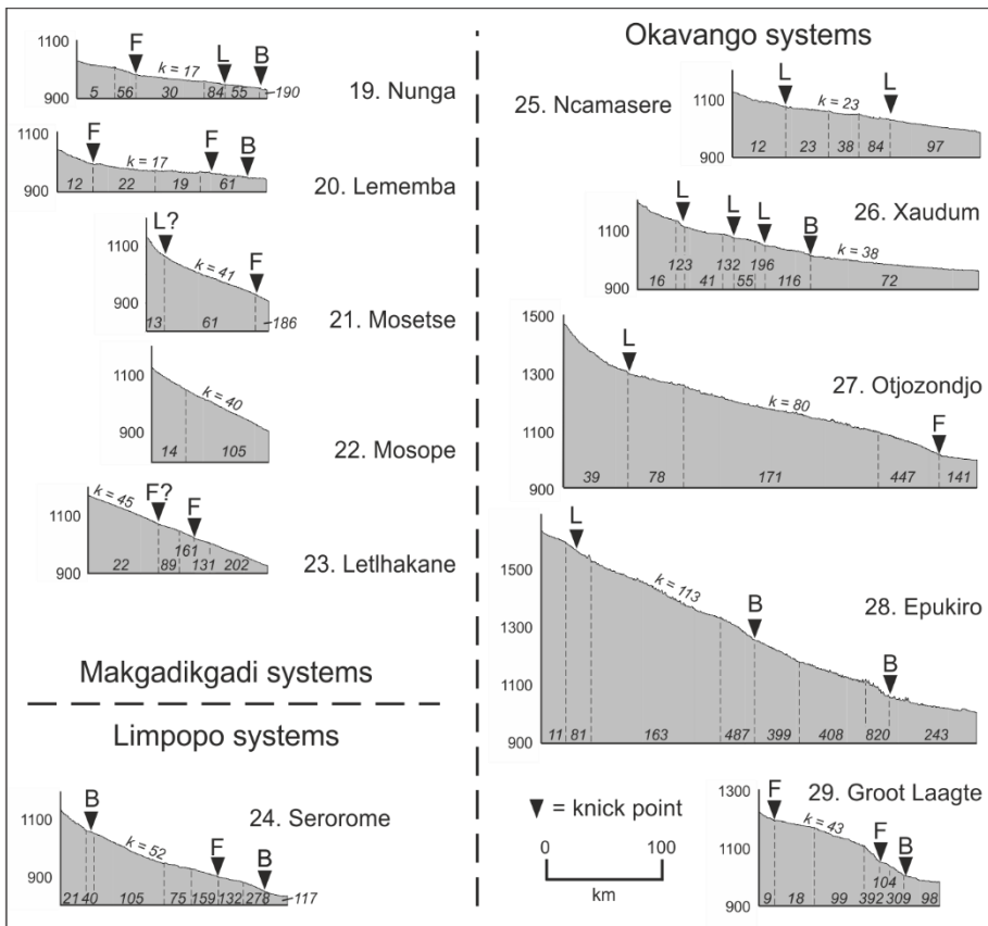
Figure 8: SRTM-derived long-profiles for the externally-draining Limpopo and internally-draining Okavango and Makgadikgadi dry valley networks (after Nash and Eckardt, 2016). See Figure 6 for further details.
