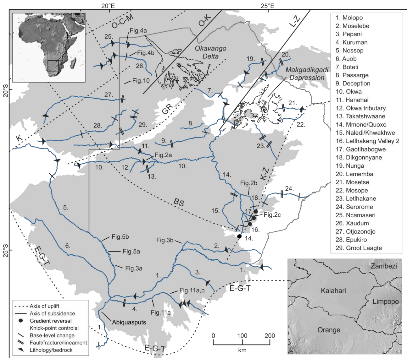
Figure 1: Major dry valley and ephemeral river systems in Botswana and the wider Kalahari Basin (after Nash and Eckardt, 2016). The Botswana border is delimited by a grey line and the area covered by Kalahari Group sediments shaded pale grey. Knickpoints and sections of valleys that exhibit gradient reversals are indicated. Knickpoints are distinguished according to their dominant control: base-level change; intersection with a fault, fracture or lineament; or differential rock resistance across a lithological boundary. The location of major flexural axes (after Haddon and McCarthy, 2005) are also shown (BS, Bakalahari Schwelle; E-G-T, Etosha-Griqualand-Transvaal axis; GR, Ghanzi Ridge; K-Z, Kalahari-Zimbabwe axis; L-Z, Luangwa-Zambezi axis; O-K, Okavango-Kafue axis; O-C-M, Otavi-Caprivi-Mweru axis; K, Khomas axis). The numbers shown against individual valley segments are used in Figures 6-8. Inset maps (derived from SRTM30 digital terrain data at 1 km resolution) indicate the area covered by the main figure in relation to Africa (top left) and the boundaries between the Okavango-Kalahari, Orange, Limpopo and Zambezi drainage basins (bottom right; note that this map covers the same geographical area as the main figure).
