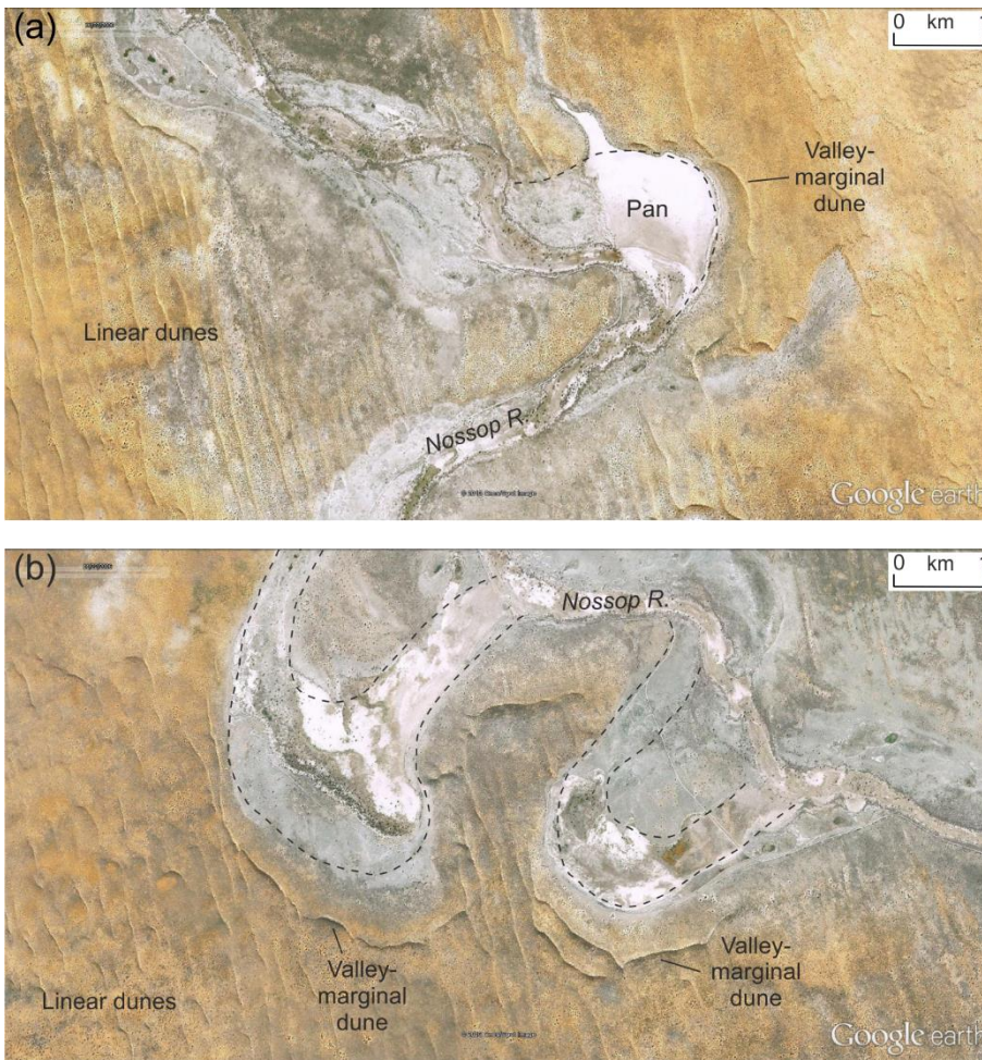
Figure 5: Abandoned meanders (dashed line) and valley floor pans along the course of the Nossop River where it forms the boundary between Botswana and South Africa. Linear dunes and valley-marginal dunes (see Bullard and Nash, 2000) are also indicated. See Figure 1 for locations of images (a) and (b). Images courtesy of Google Earth (date of images, 22 November 2006).
