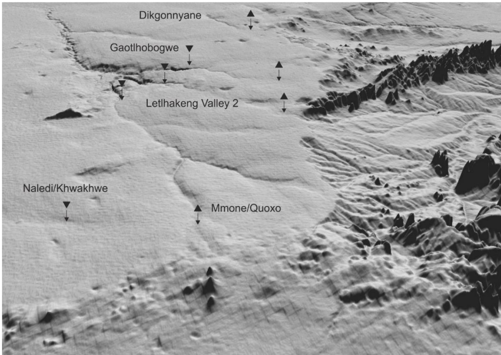
Figure 9: Oblique SRTM-derived view of the headwaters of the Mmone/Quoxo system, showing areas of gradient reversal and major knickpoints (looking NNE; field of view approximately 70 km wide) (after Nash and Eckardt, 2016). Inverted black triangles indicate the position of the knickpoints in the Dikgonnyane, Gaotlhobogwe, Letlhakeng Valley 2, Mmone/Quoxo and Naledi/Khwakhwe systems shown in Figures 1 and 7. Upright black triangles mark the approximate positions of the gradient reversals in the headwater sections of the Dikgonnyane, Gaotlhobogwe, Letlhakeng Valley 2, and Mmone/Quoxo systems. The smooth terrain on the left of the image is blanketed with Kalahari Group sediments, whilst the more dissected terrain to the right marks the western edge of the Limpopo catchment. The image demonstrates the indistinct nature of the drainage divides between Kalahari valley systems.
