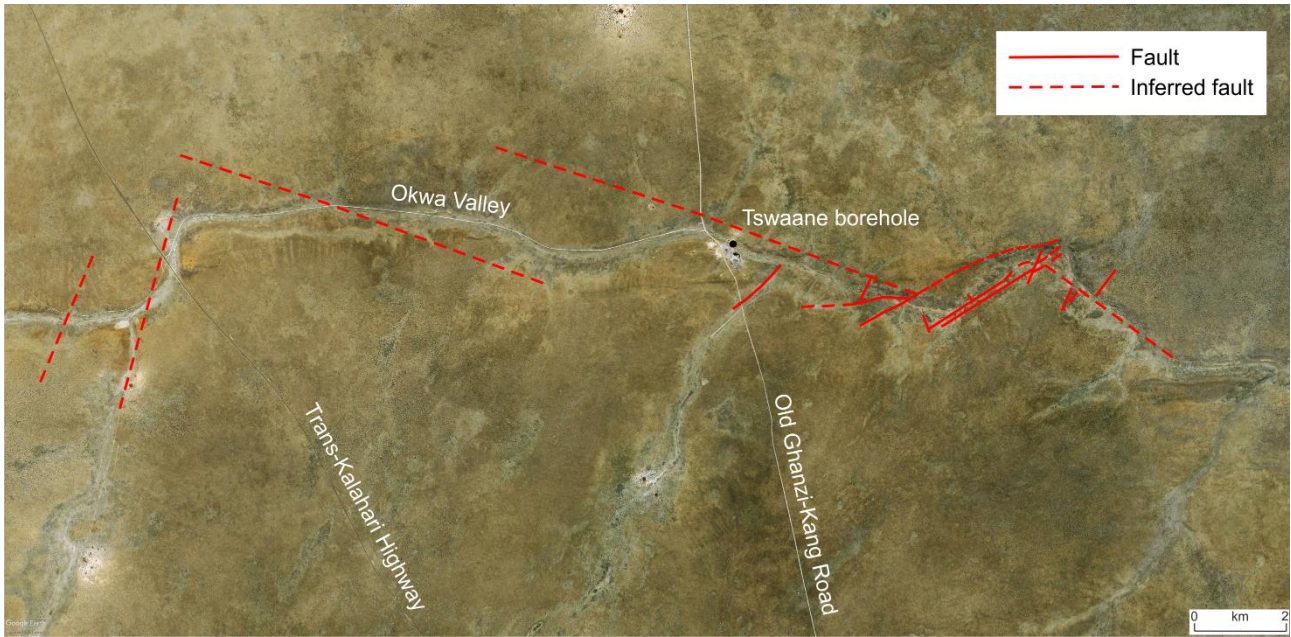
Figure 12: Fault-controlled section of the Okwa Valley close to Tswaane borehole. Approximate positions of faults shown as red lines, dashed when inferred. Fault patterns redrawn after Aldiss and Carney (1992) and Ramokate et al. (2000).
