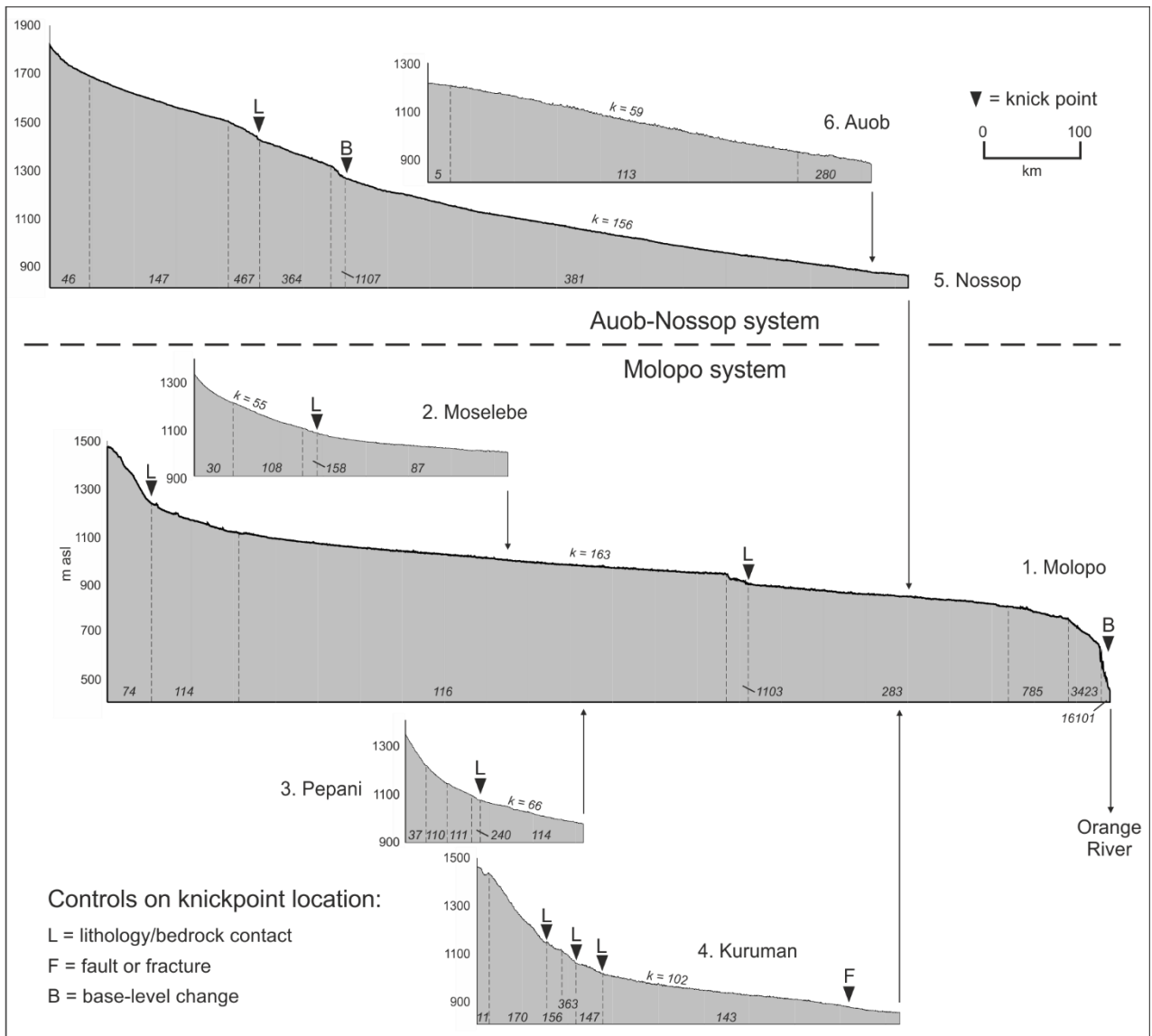
Figure 6: SRTM-derived long-profiles for the externally-draining Southern Kalahari dry valley networks (after Nash and Eckardt, 2016). Stream gradient index ( k ) values are shown for comparative purposes for entire long-profiles and individual valley segments. Stream gradient indices were calculated using the equation: k = (H_i - H_j) / (\ln L_j - \ln L_i) where H is altitude and L the horizontal distance between two points i and j (after Hack, 1973). Vertical arrows indicate confluence points between valley segments and the connection with the Orange River. Long-profiles are plotted at the same horizontal scale in Figures 5-7, with 250-times vertical exaggeration. See Figure 1 for locations of valley segments.
