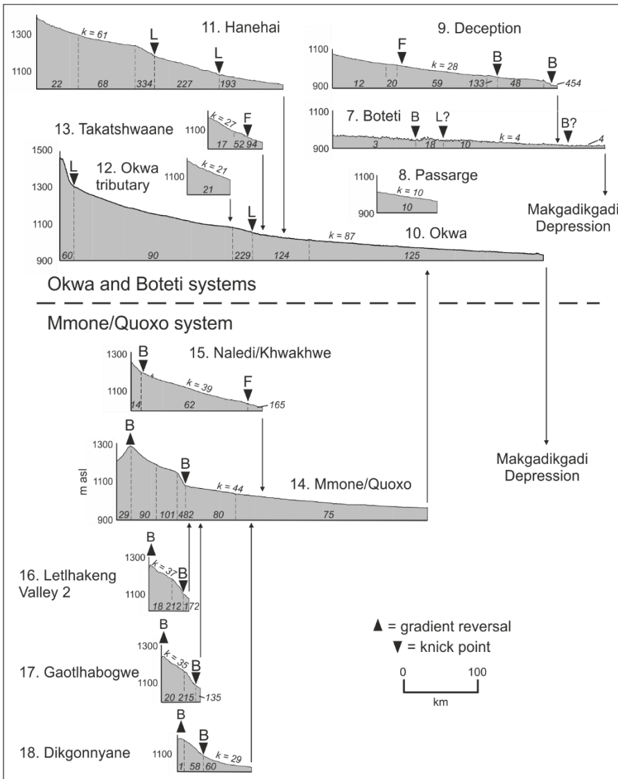
Figure 7: SRTM-derived long-profiles for the internally-draining Okwa and Mmone/Quoxo dry valley networks (after Nash and Eckardt, 2016). The profile for the ephemeral Boteti River is shown for comparison. See Figure 6 for further details.
