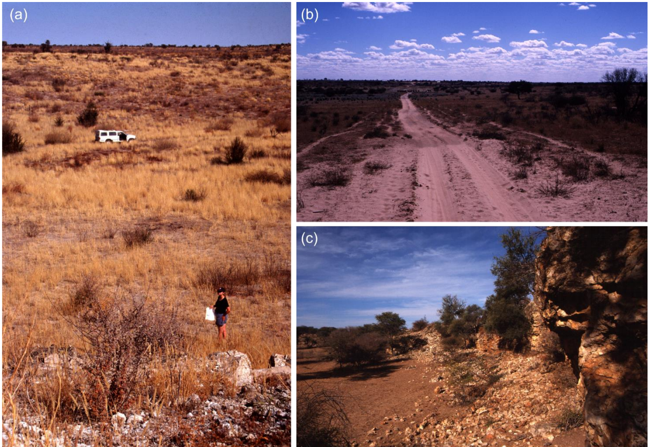
Figure 2: Views of internally-draining (endoreic) dry valleys in Botswana: (a) Okwa valley immediately west of Tswaane borehole; (b) Dikgonnyane valley; (c) Gaotlhobogwe valley immediately downstream of the major knickpoint ~60 km from the valley headwater area (see Figures 1 and 7) with exposures of silcrete (photographs: David Nash).
